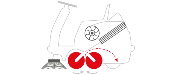
Tandem-Walzen-System (TRS)
