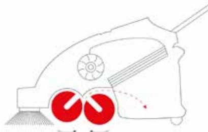
Tandem-Walzen-System (TRS)
